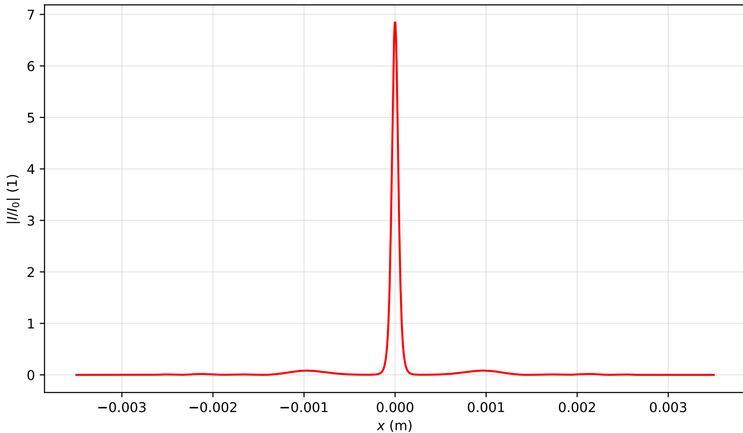
Intensity profile I(x, y = 0, z = 0.796)/I_0 , P_{in}=8.0P_{cr} , artificial time
